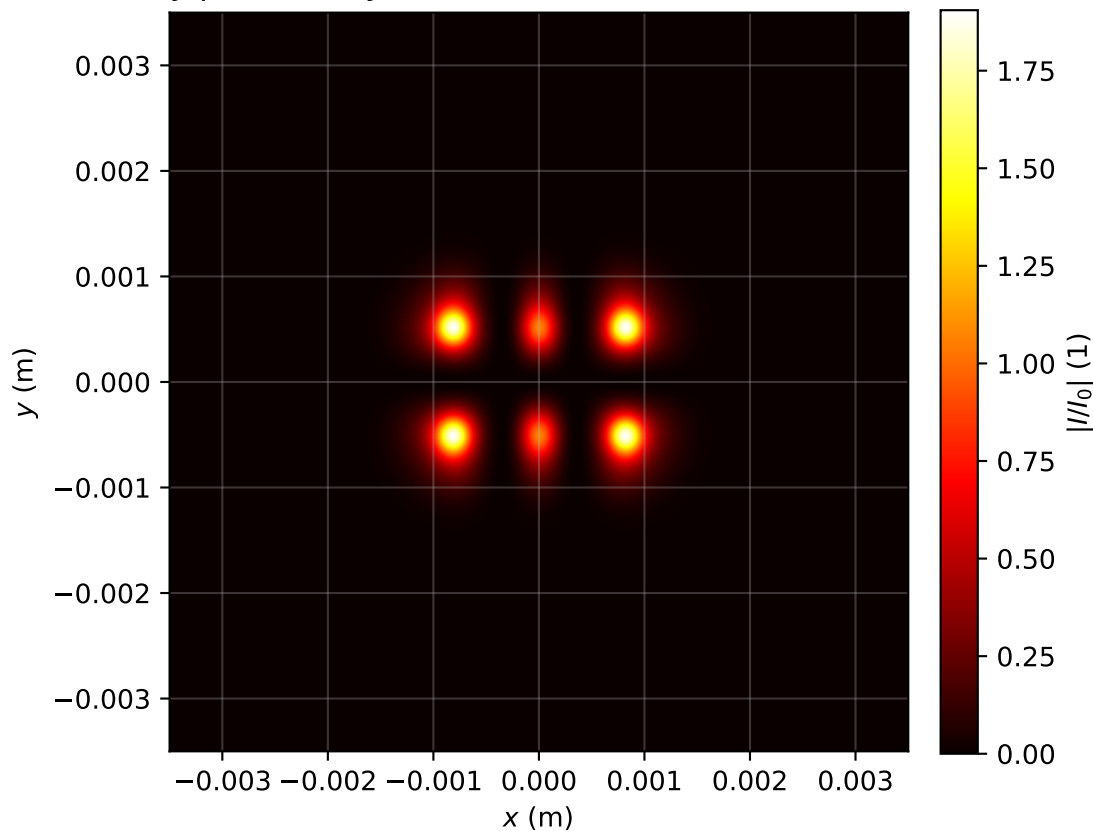
Intensity profile I(x, y, z = 0.398)/I_0 , P_{in}=5.0P_{cr} , artificial time
